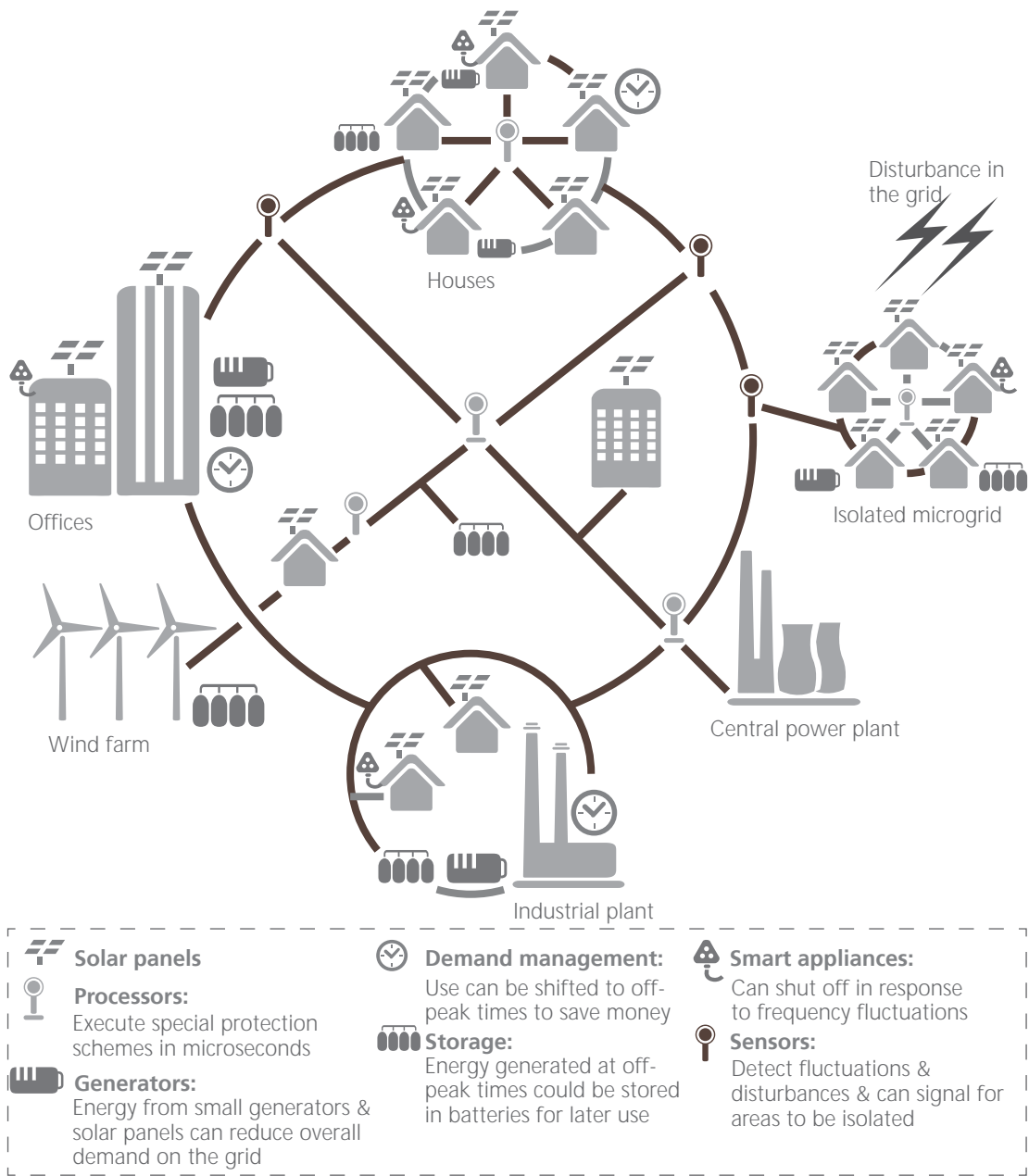
Figure 2.24 Smart Grid
