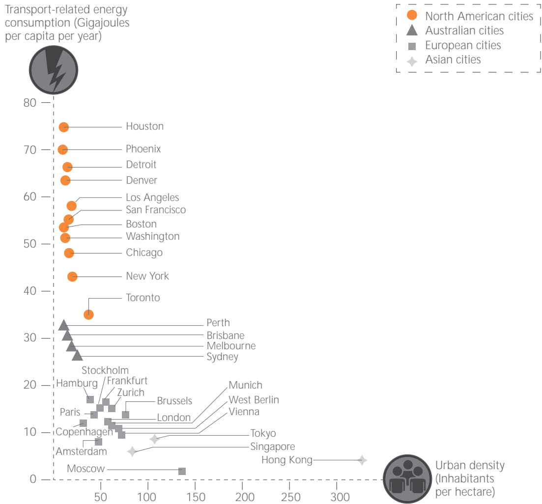
Figure 1.9 Urban Density and Transport Related Energy Consumption
